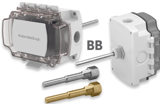
Polycarbonate BB (IP66, NEMA 4X)
