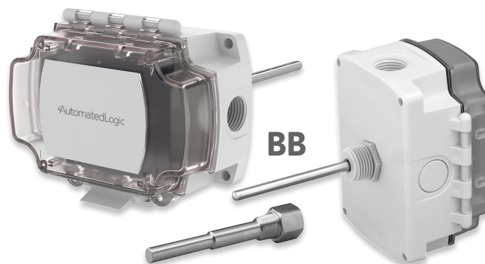
Polycarbonate BB (IP66, NEMA 4X)
