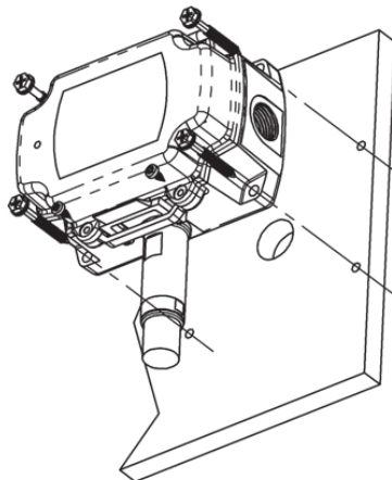
Outside Humidity in a BBox (BB) Enclosure
